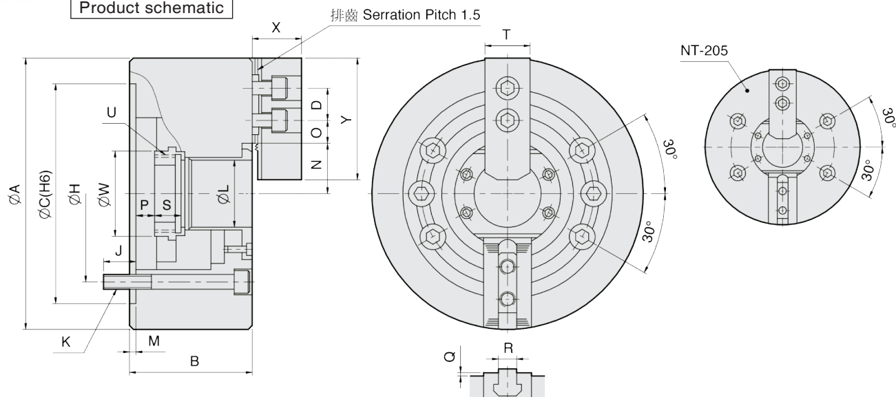
Product schematic
