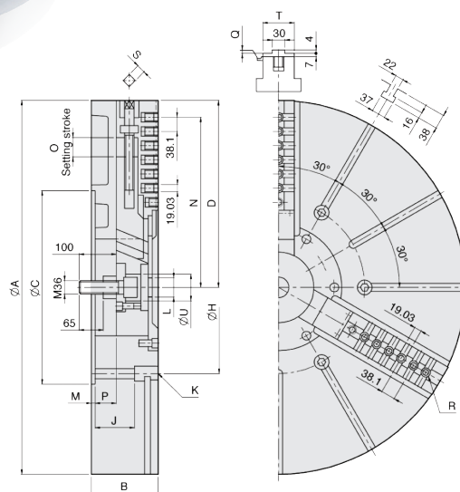
Soft jaw HC40-1
