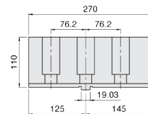
Soft jaw HC40-1
