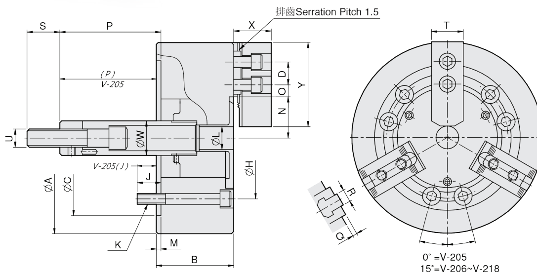
Product schematic
