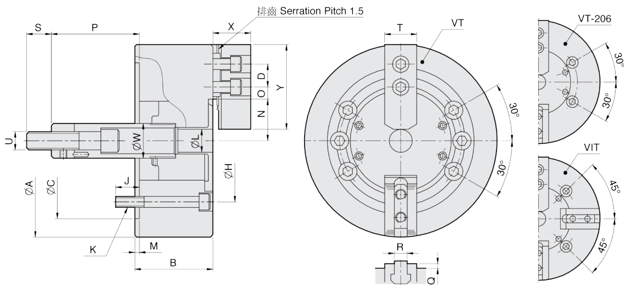
Product schematic
