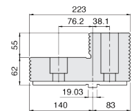
Hard jaw HJ40-1
