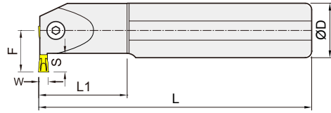
Steel shank (right shown) 鋼柄 右向示意圖
