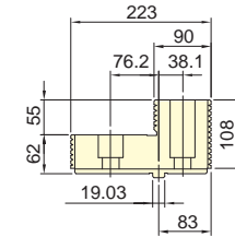
硬爪 Hardened jaw HJ-40~79
