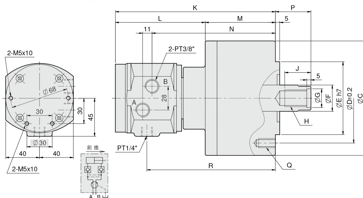
Product schematic
