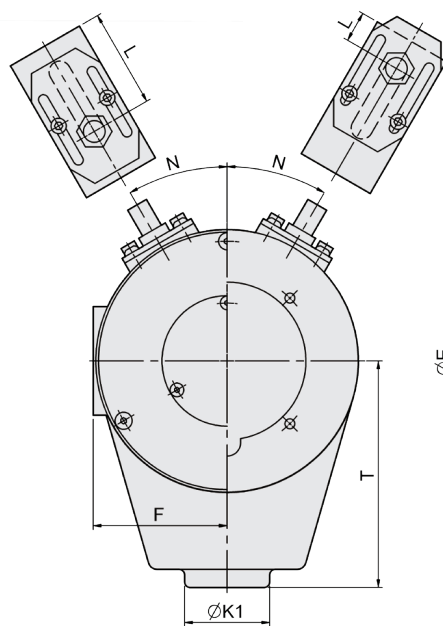
Product schematic
