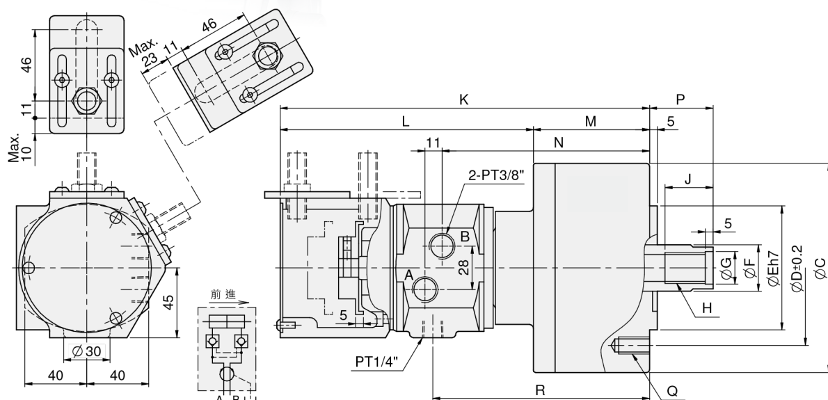
Product schematic
