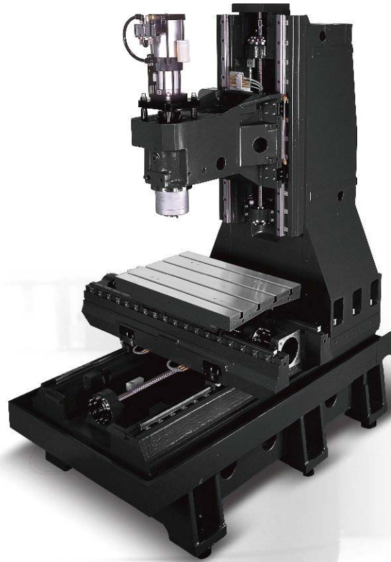
CNV-550 / 750 structure
