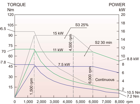
MITSUBISHI 15HP Model : 550 / 750 / 850 / 1050 / 1100 / 1300
