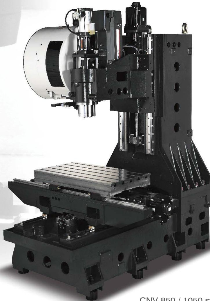
CNV-850 / 1050 structure
