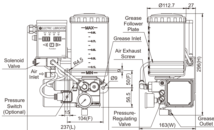
Dimensional Drawing of KGNB-35-2-C-5-0-PC
