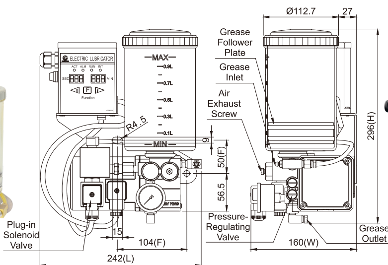
Dimensional Drawing of KGNB-35-2-C-5-1
