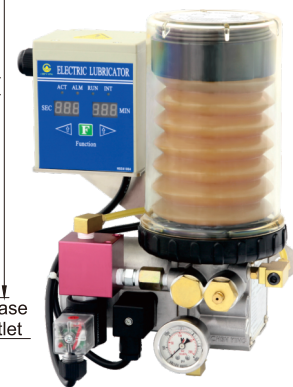
KGNBP-07-2-C-5-1 with Grease Cartridge (Electric Type)
