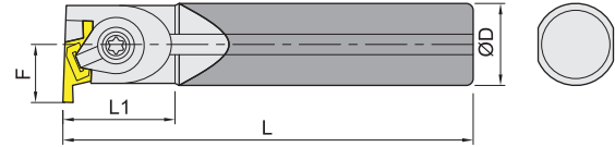
Carbide shank (right shown) 鎢鋼柄 右向示意圖
