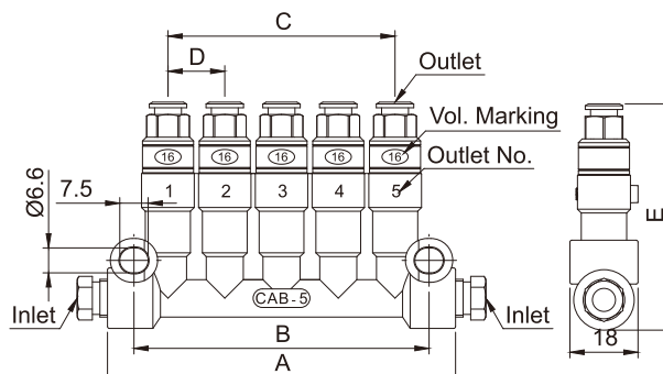
Dimensional Drawing of CAB-5-B-22222-AA
