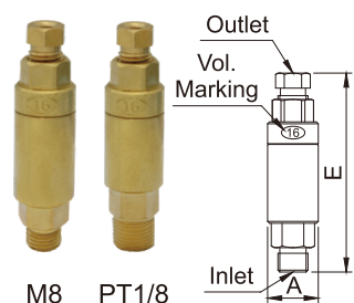
CAB-1B-A-4 and CAB-1A-A-4
