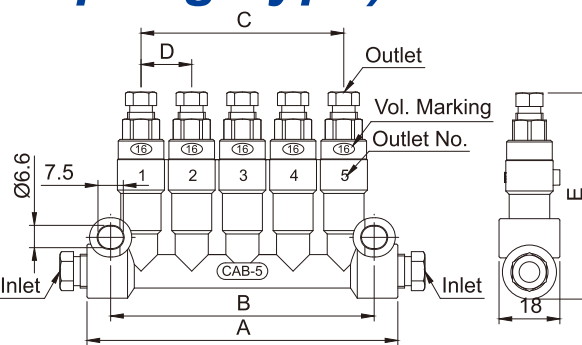
Dimensional Drawing of CAB-5-A-44444-AA
