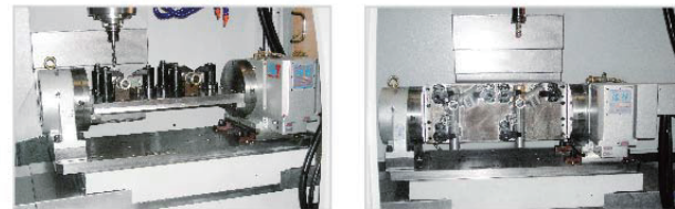
(Example of workpiece installation)
