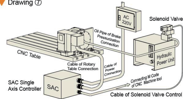
▼ Drawing ⑦
