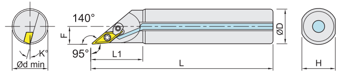
Coolant steel shank+clamp (right shown)
