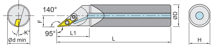
Coolant carbide shank+clamp (right shown)
