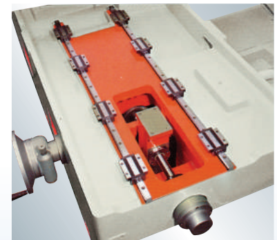
Lower Slide Way is equipped with Heavy Bearing, Linear Motion System and Ball Screws.
