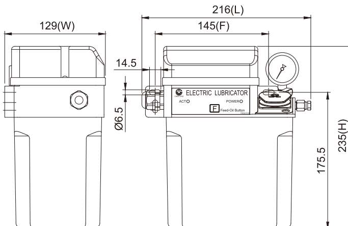
Dimensional Drawing of CESG03-01-C-3
