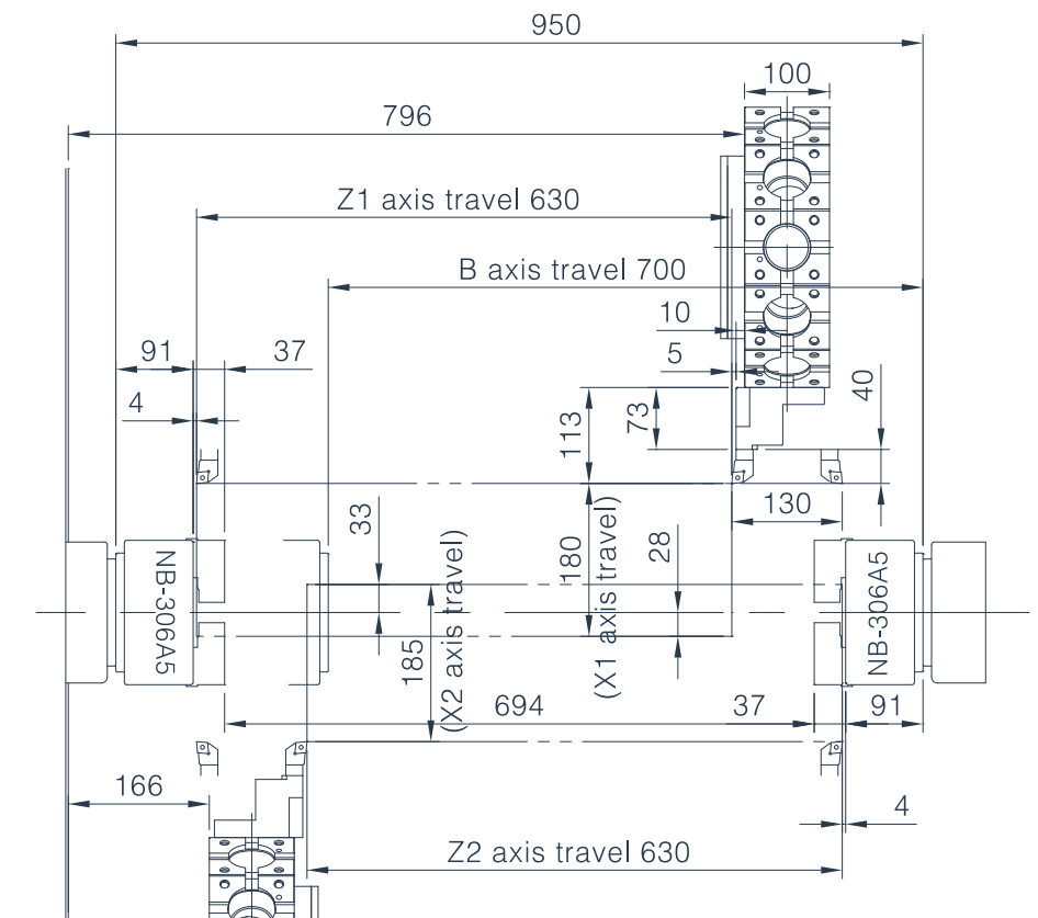
Single OD Tool Holder
