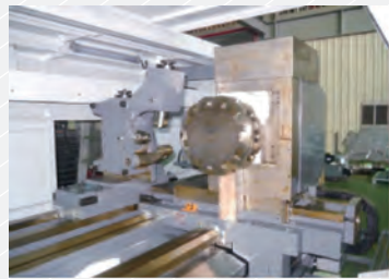
Driving tool with Y axis + spindle with CS / CF (option) is available.
