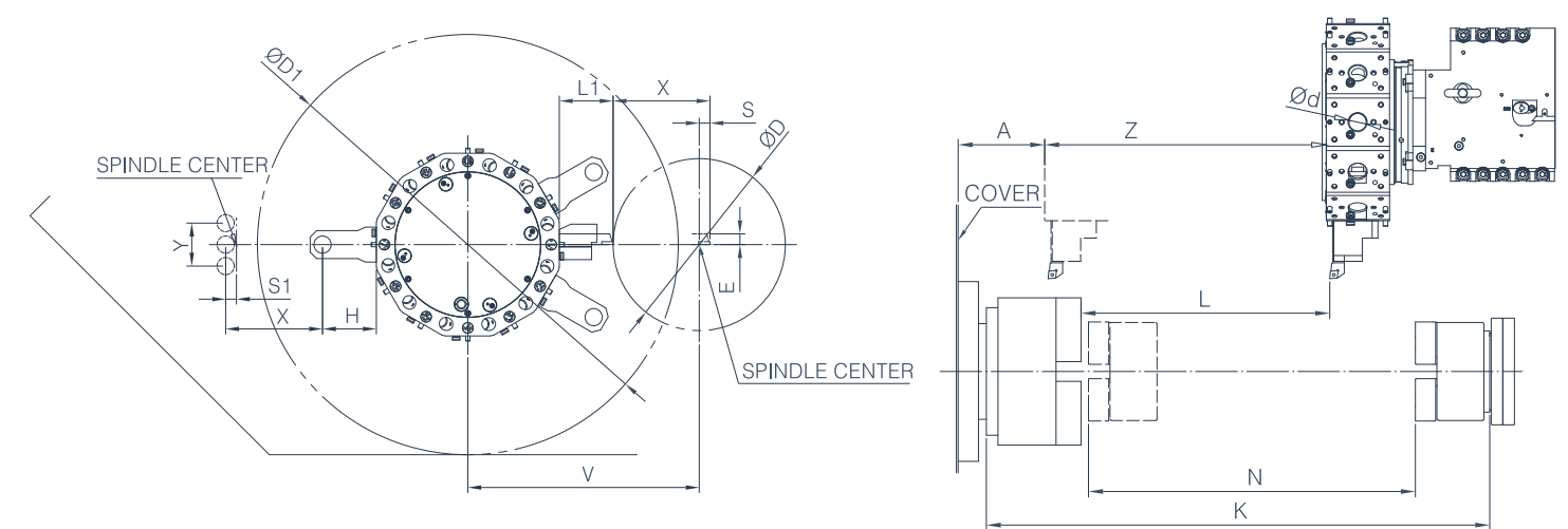
POWER TURRET / TWIN SPINDLE / Y AXIS VDI RADIAL MOUNTING OPT.
