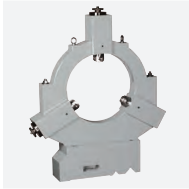
STEADY REST
