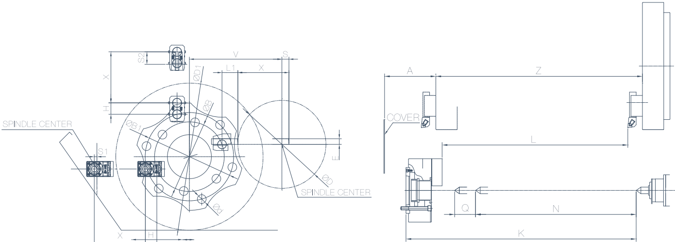
POWER TURRET VDI AXIAL MOUNTING OPT. UNIT:mm
