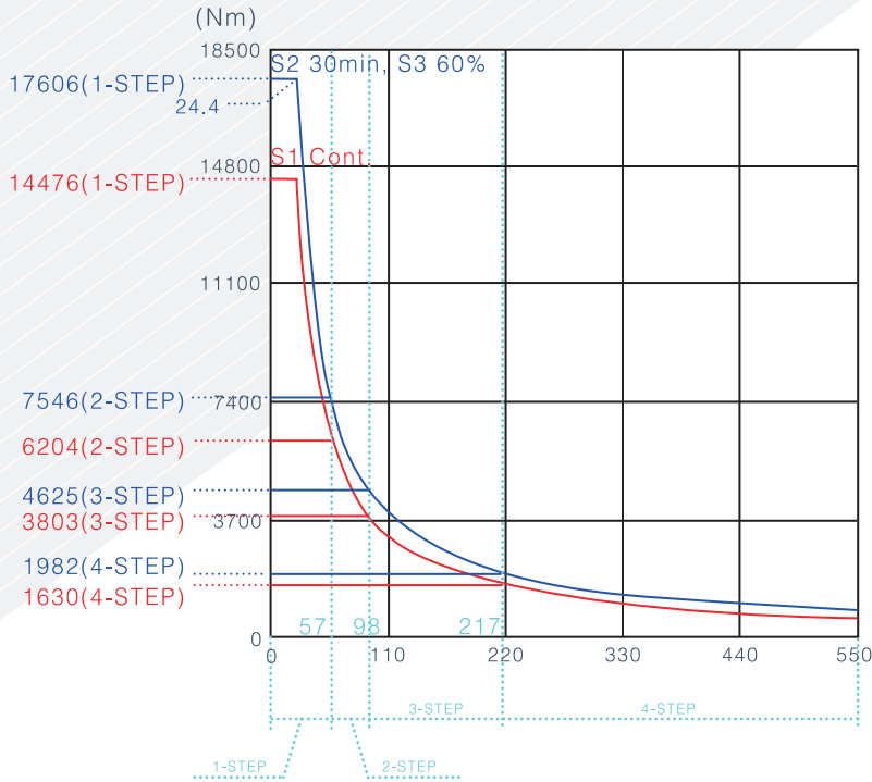
SPINDLE SPEED (rpm)
