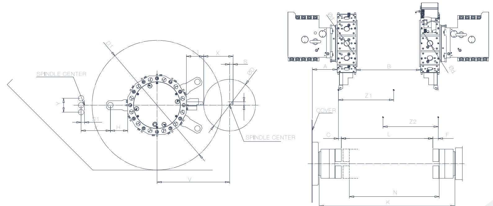
POWER TURRET / TWIN SPINDLE / TWIN TURRET / Y AXIS RADIAL MOUNTING OPT.
