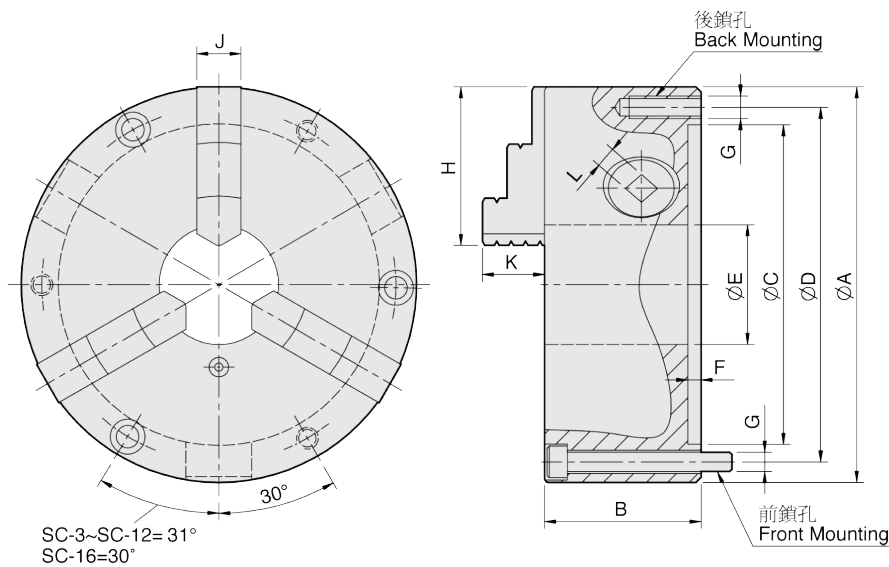
Product schematic
