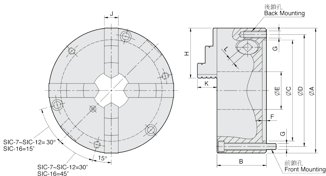
Product schematic
