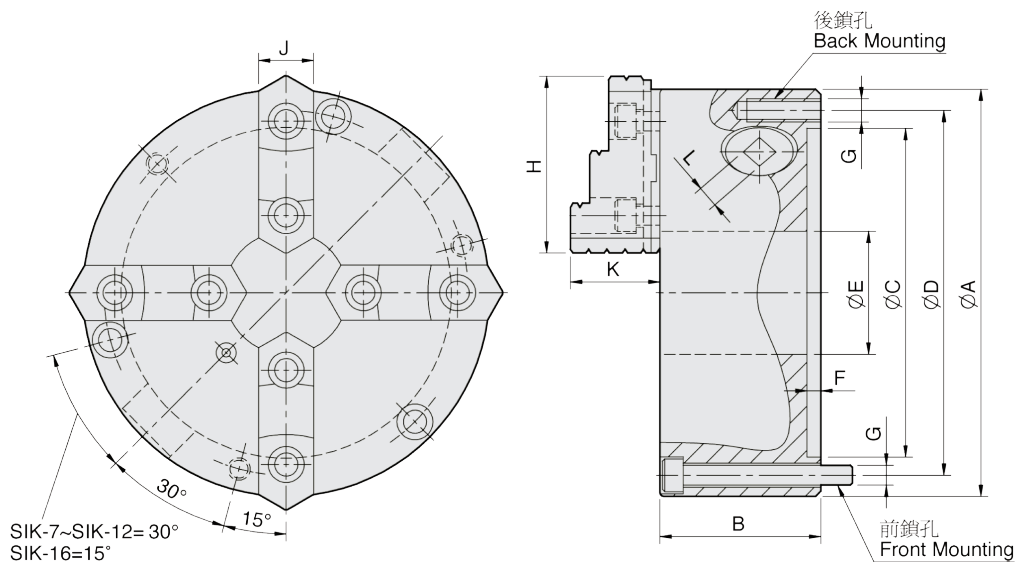
Product schematic
