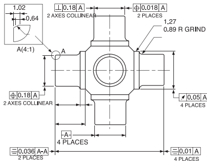
JHC-18S-CNC4 軸撞球研磨
